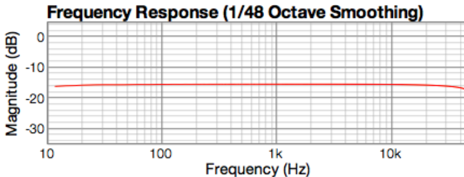
KCM, -15dBu out Into 1.5K load ■
