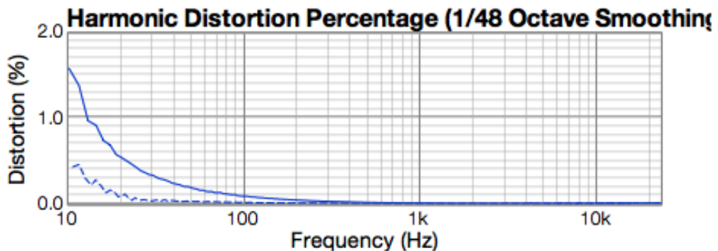
KCM, -15dBu out Into 1.5K load ■
